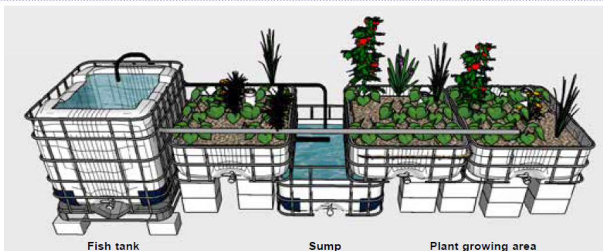
Figure 44: Adaptation of the RAS into an Aquaponics System
