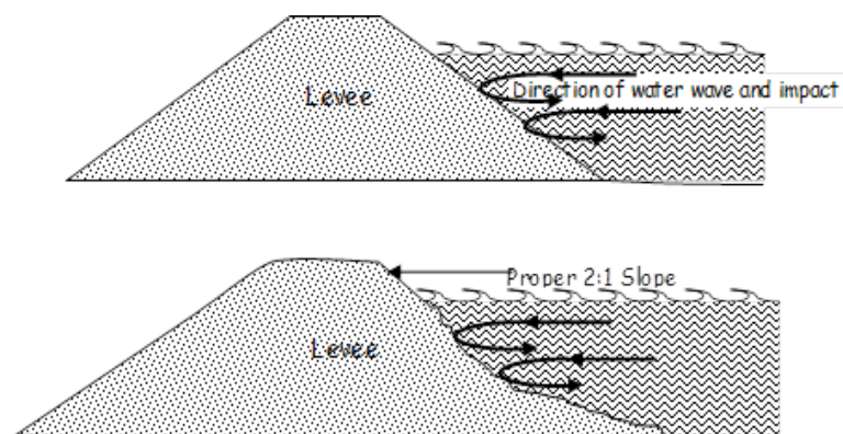
Figure 18: Impact of wave action on pond walls.
